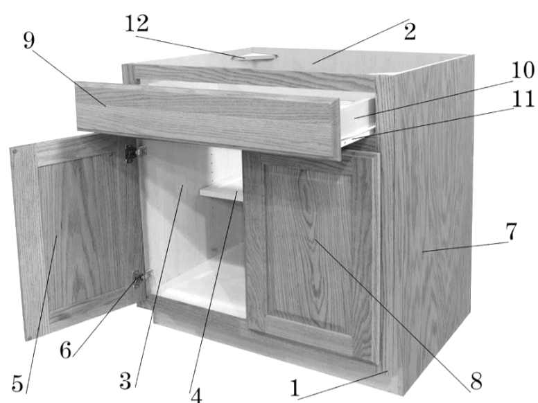
BASE CABINET
